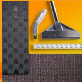
Tools and products required to install using Self Lock adhesive tiles.
